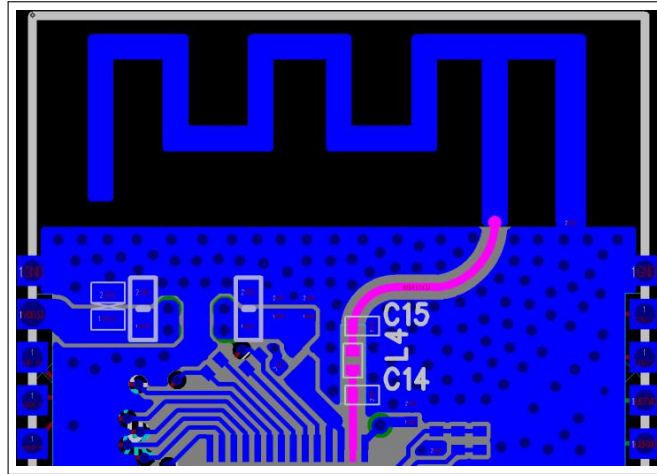
Figure 17: ESP32 RF Layout in a Four-layer PCB Design
