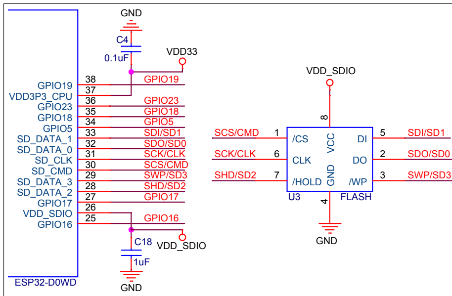
Figure 4: ESP32 Flash
